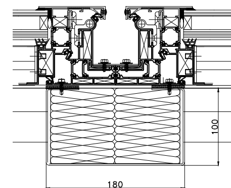
DETAIL CHENEAU
